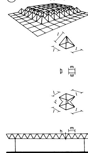
⑭ Space frame system
